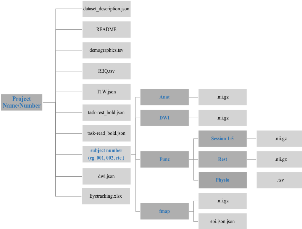
Figure 3. Organization of File Directory and Data Structure (Folder names are in blue, and file names are in black.)
